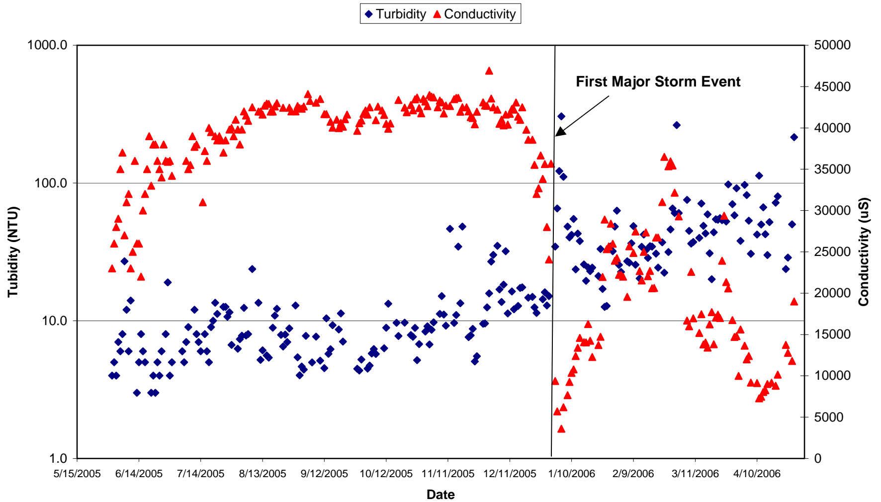
Figure 1.1 MMWD Seawater Desalination Pilot Program Source Water Daily Turbidity and Conductivity
