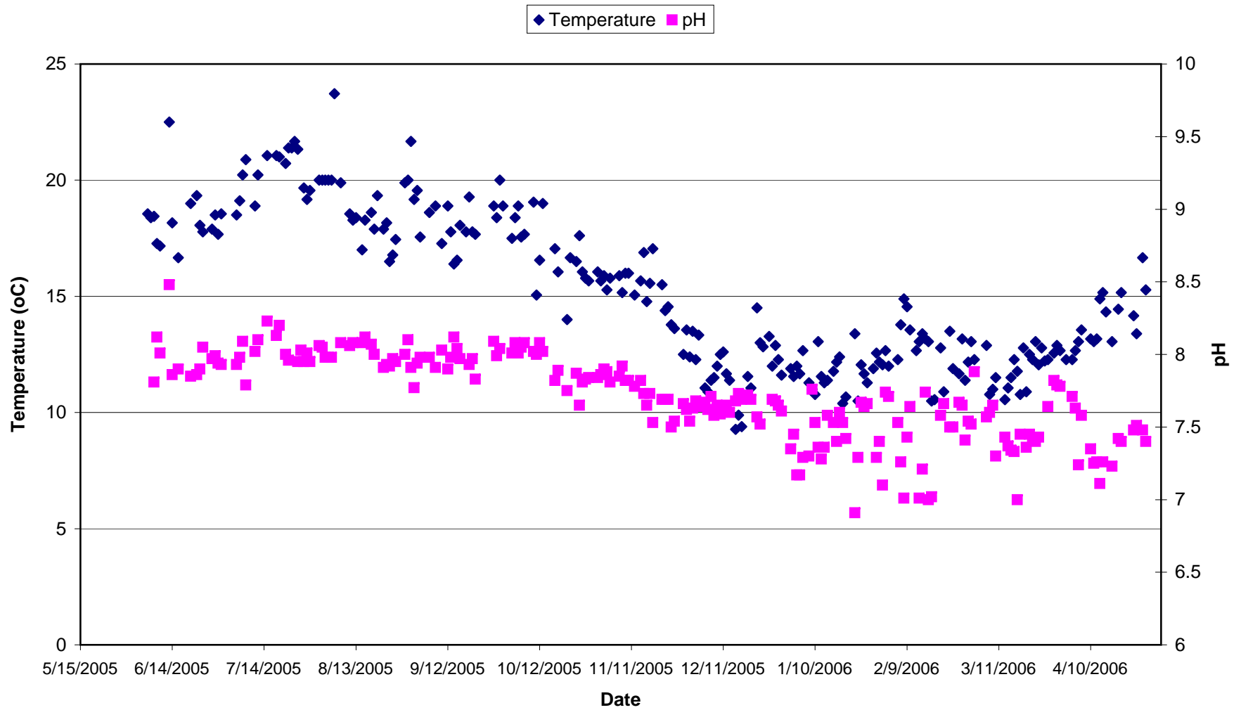
Figure 1.2 MMWD Seawater Desalination Pilot Program Source Water Daily Temperature and pH
