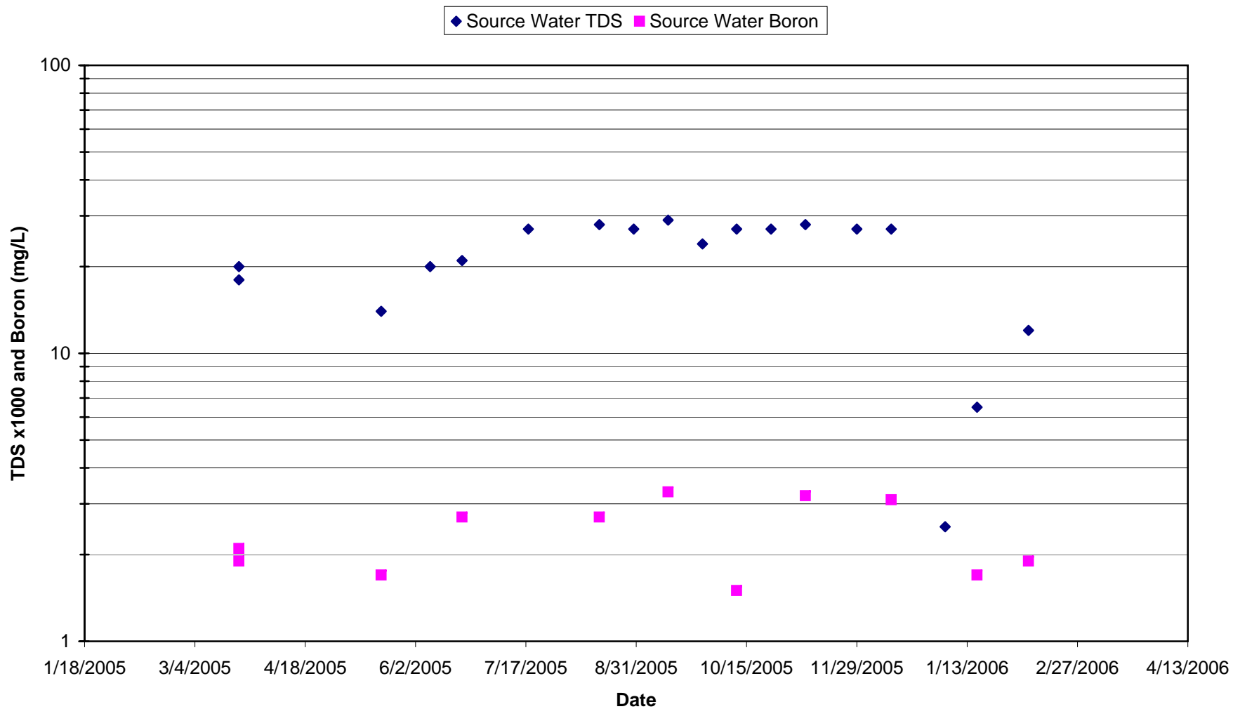
Figure 1.3 MMWD Seawater Desalination Pilot Program Source Water Total Dissolved Solids and Boron
