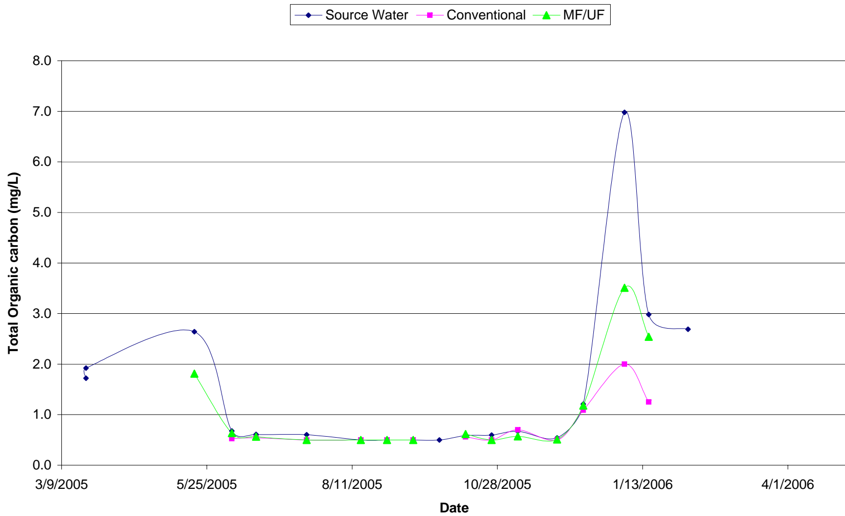
Figure 1.4 MMWD Seawater Desalination Pilot Program Source Water and Filtrate Total Organic Carbon (TOC) Levels
