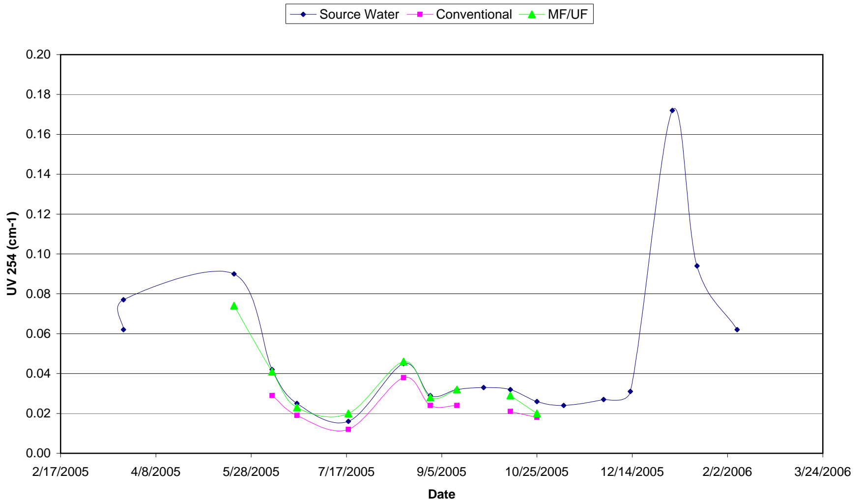
Figure 1.5 MMWD Seawater Desalination Pilot Program Source Water and Filtrate UV 254 Levels
