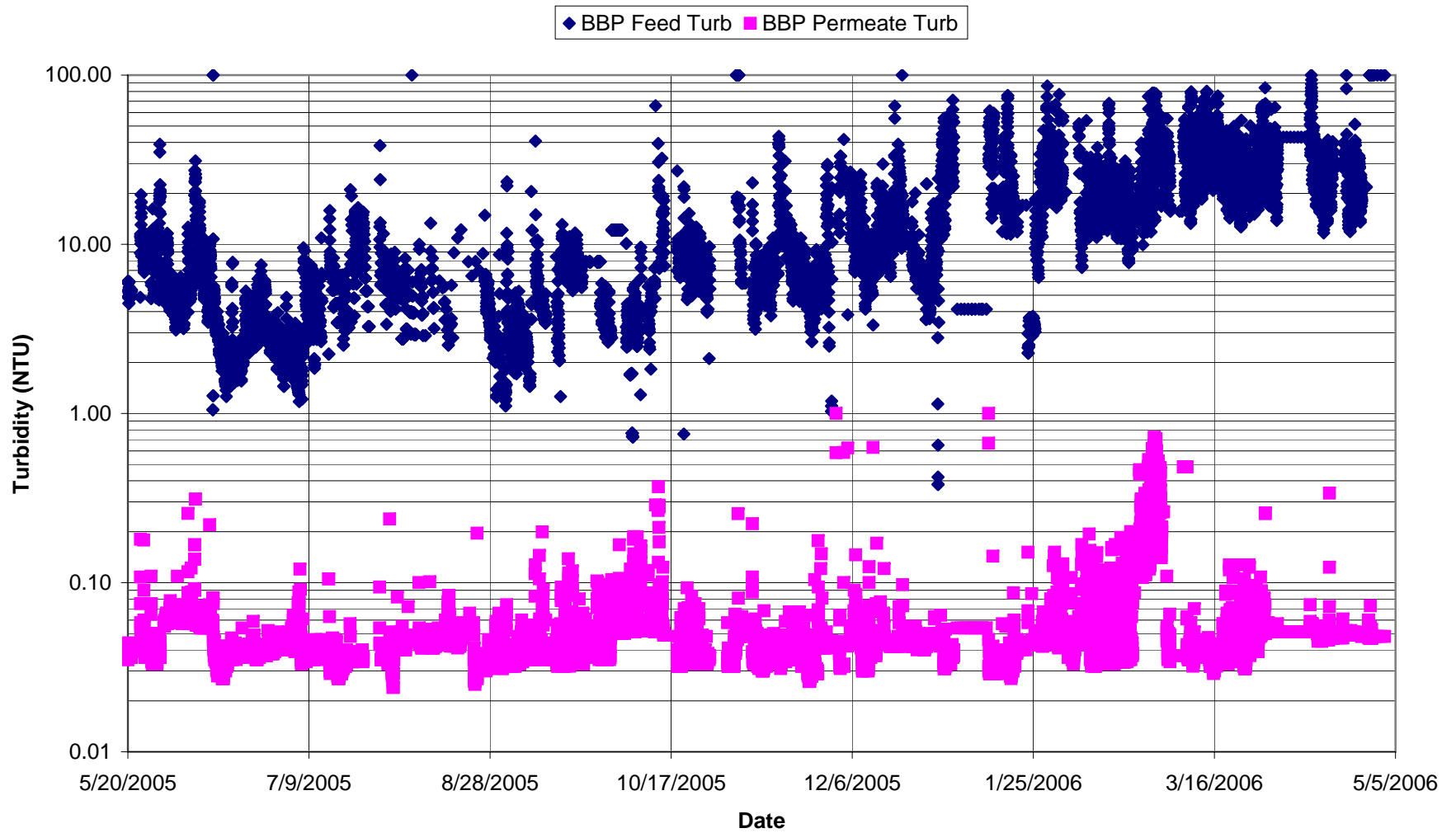
Figure 2.1 MMWD Seawater Desalination Pilot Program UF System Feed and Filtrate Turbidity
