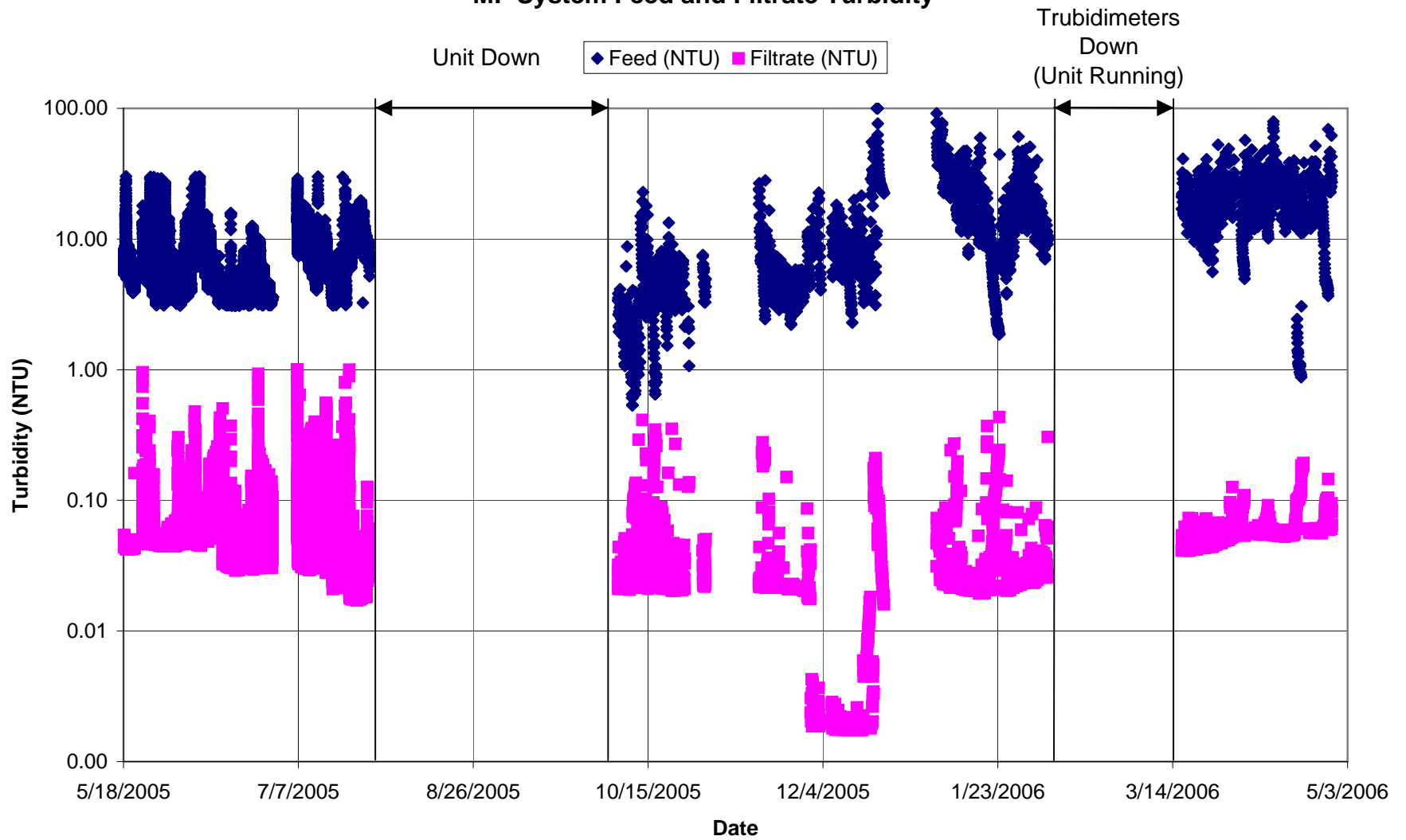
Figure 2.3 MMWD Desalination Pilot Program MF System Feed and Filtrate Turbidity
