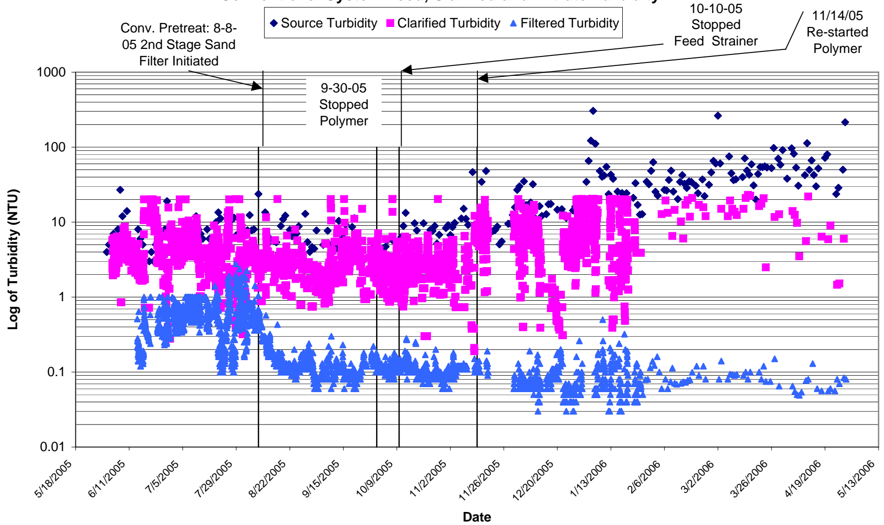
Figure 3.1 MMWD Seawater Desalination Pilot Program Conventional System Feed, Clarified and Filtrate Turbidity
