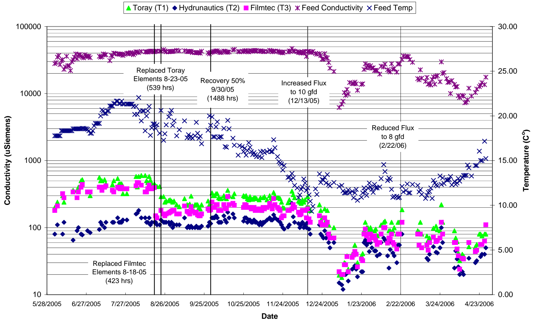
Figure 5.2 MMWD Seawater Desalination Pilot Program SWRO #2 Feed and Permeate Conductivity and Feed Temperature
