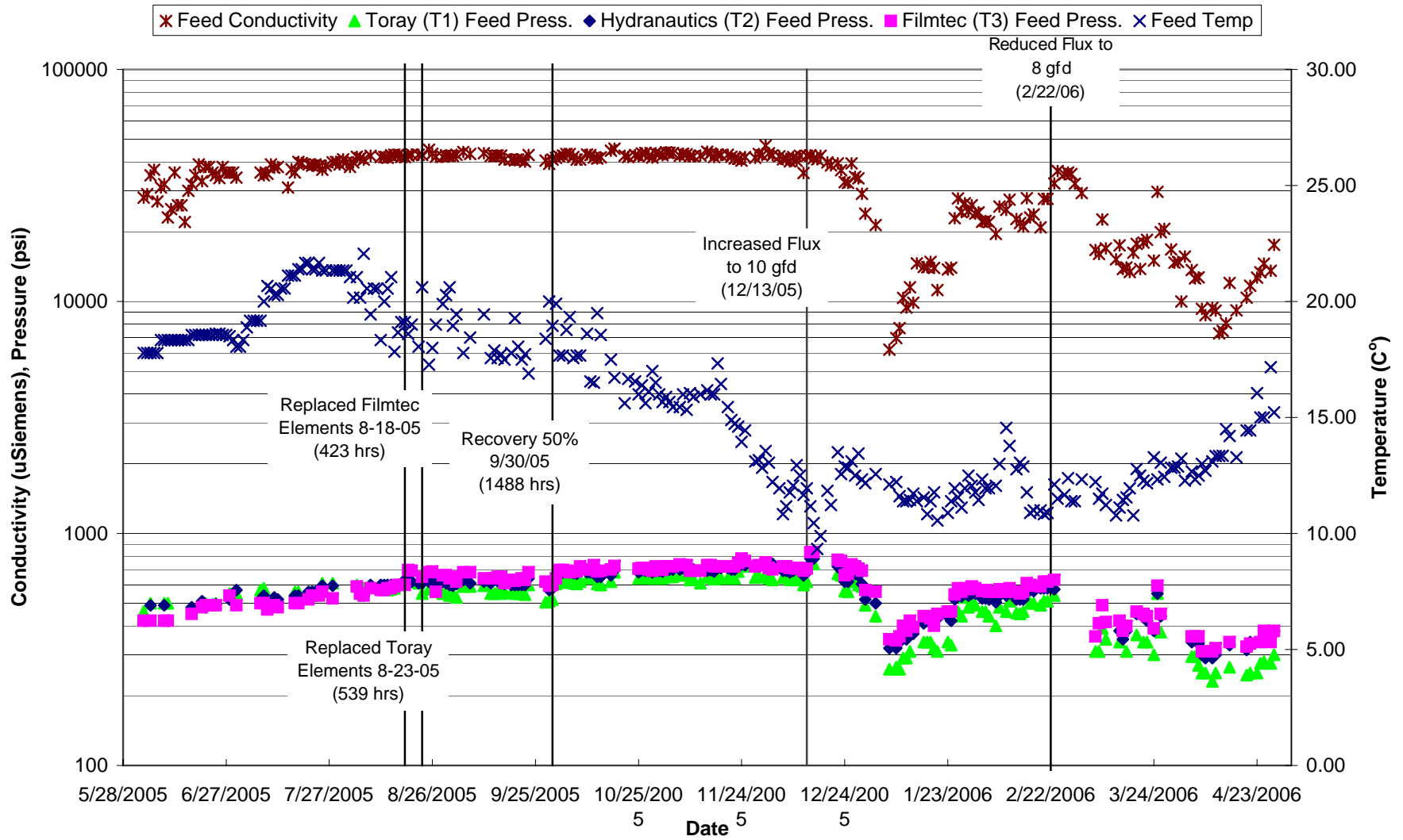
Figure 5.3 MMWD Seawater Desalination Pilot Program SWRO #2 Daily Feed Conductivity, Feed Pressure and Feed Temp.
