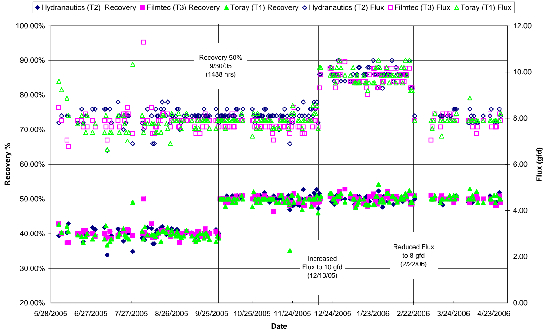
Figure 5.4 MMWD Seawater Desalination Pilot Program SWRO #2 Flux and Recovery
