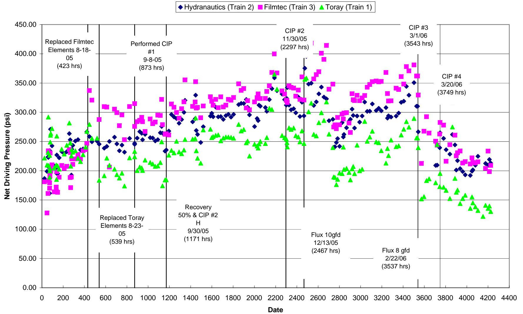
Figure 5.5a MMWD Seawater Desalination Pilot Program SWRO #2 Net Driving Pressure
