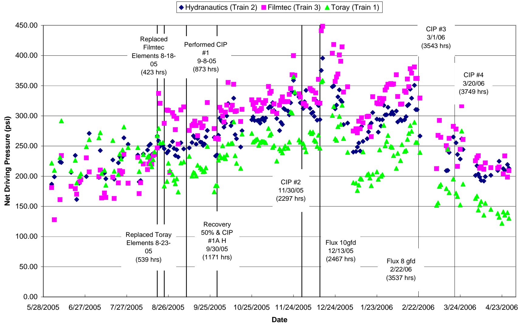
Figure 5.5 MMWD Seawater Desalination Pilot Program SWRO #2 Net Driving Pressure
