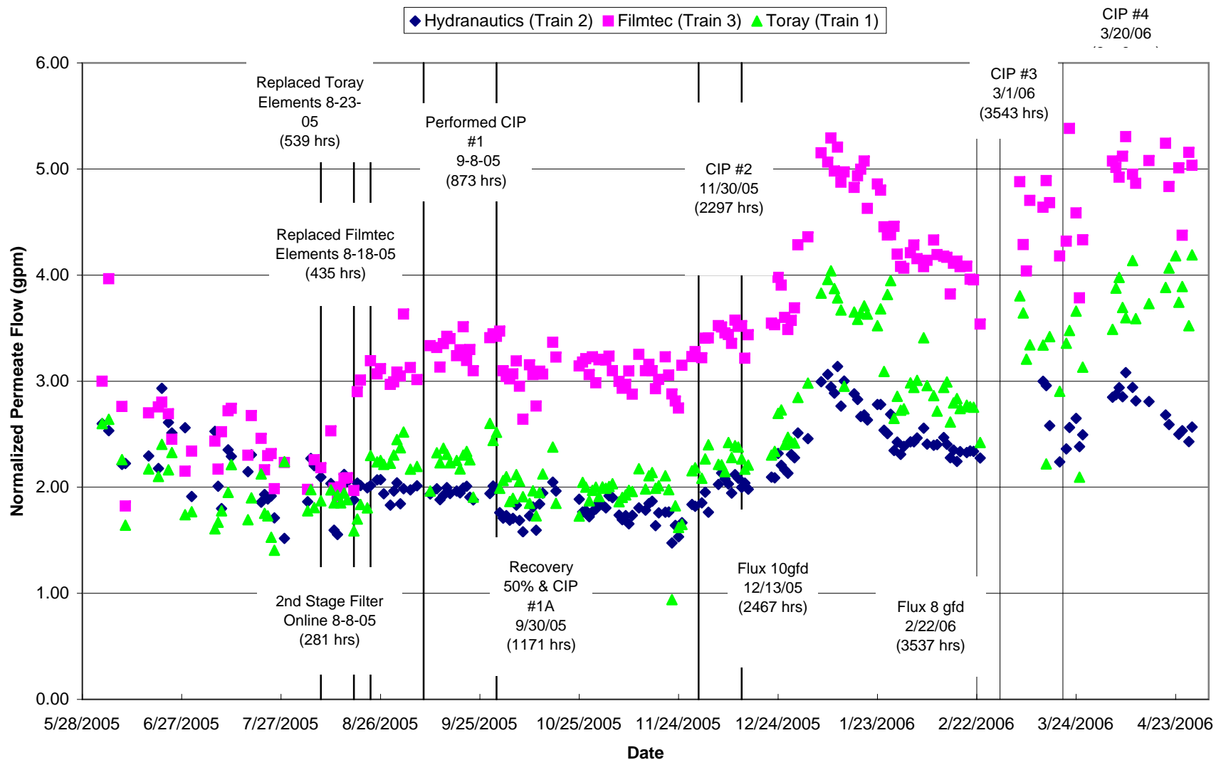
Figure 5.6 MMWD Seawater Desalination Pilot Program SWRO #2 Normalized Permeate Flow
