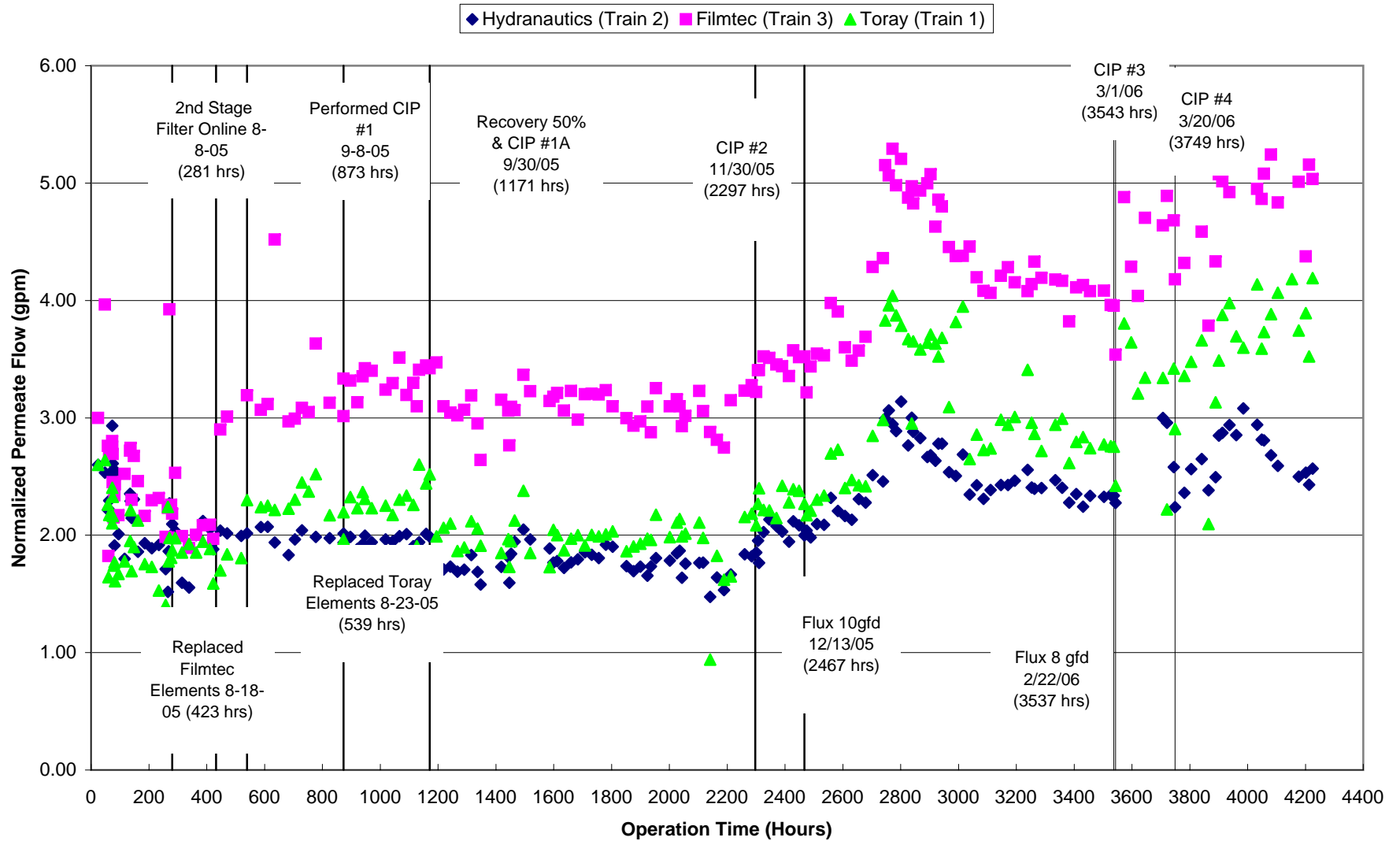
Figure 5.6a MMWD Seawater Desalination Pilot Program SWRO #2 Normalized Permeate Flow
