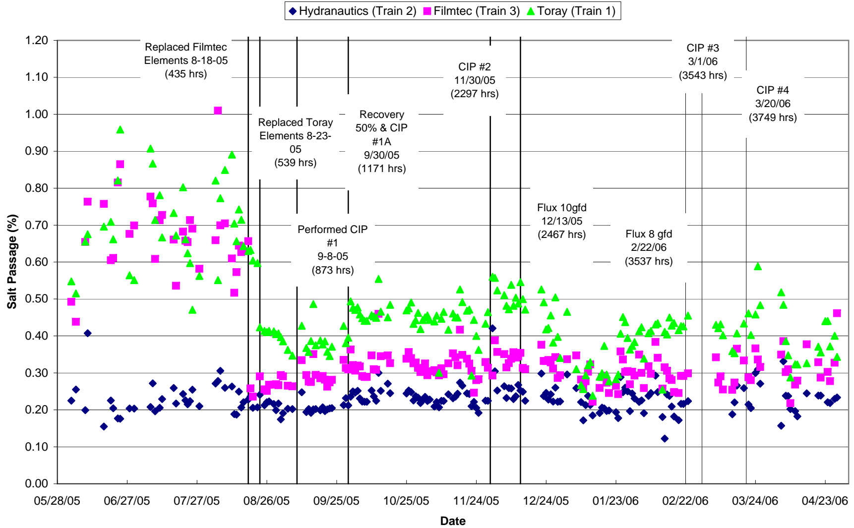
Figure 5.7.1 MMWD Seawater Desalination Pilot Program SWRO #2 Normalized Salt Passage
