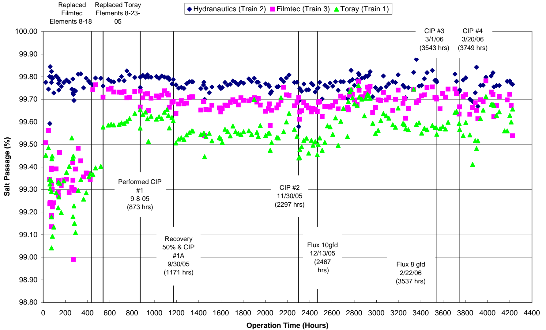
Figure 5.7a MMWD Seawater Desalination Pilot Program SWRO #2 Normalized Salt Rejection
