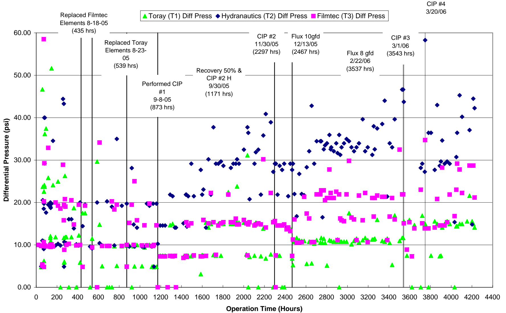
Figure 5.8a MMWD Seawater Desalination Pilot Program SWRO #2 Normalized Differential Pressure
