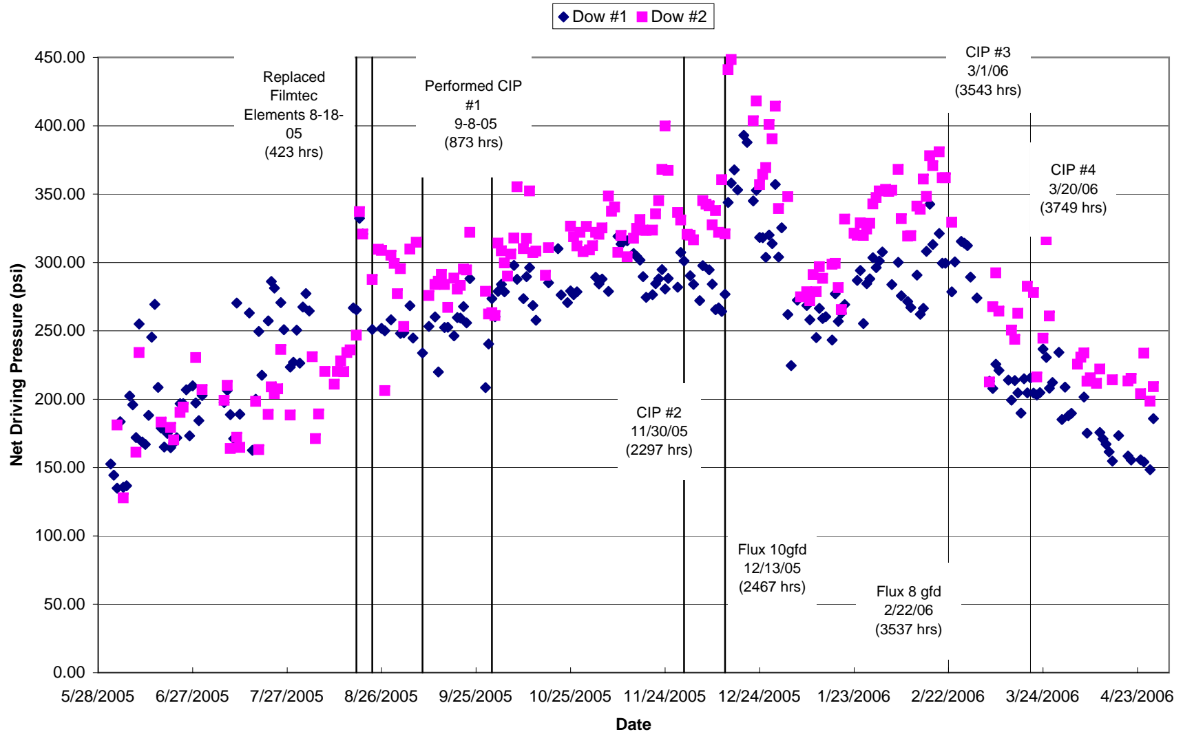
Figure 6.5 MMWD Seawater Desalination Pilot Program SWRO #1 & SWRO #2 Dow FilmTec Net Driving Pressure
