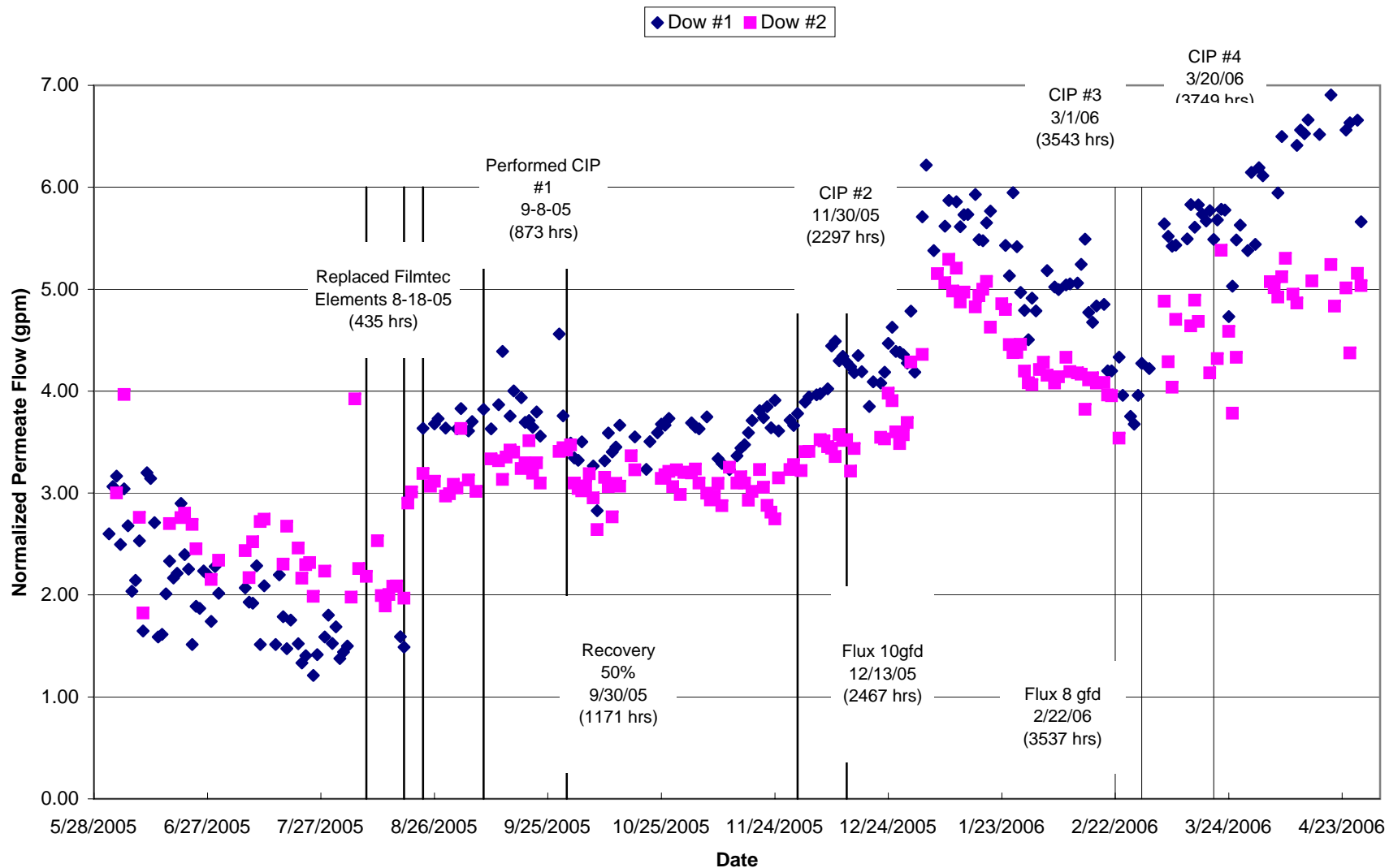
Figure 6.6 MMWD Seawater Desalination Pilot Program SWRO #1 & SWRO #2 Dow FilmTec Normalized Permeate Flow
