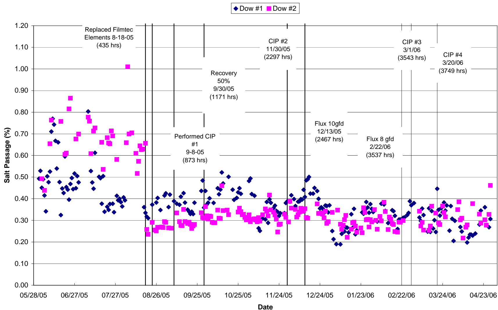
Figure 6.7.1 MMWD Seawater Desalination Pilot Program SWRO #1 & SWRO #2 Dow FilmTec Normalized Salt Passage
