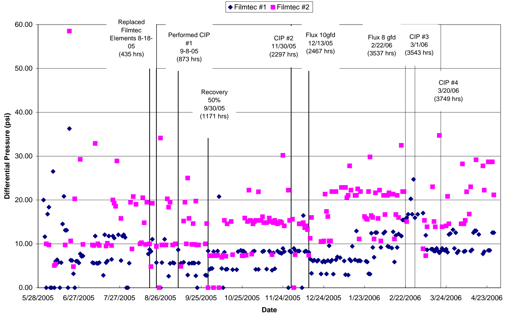
Figure 6.8 MMWD Seawater Desalination Pilot Program SWRO #1 & SWRO #2 Dow FilmTec Normalized Feed/Brine Differential Pressure
