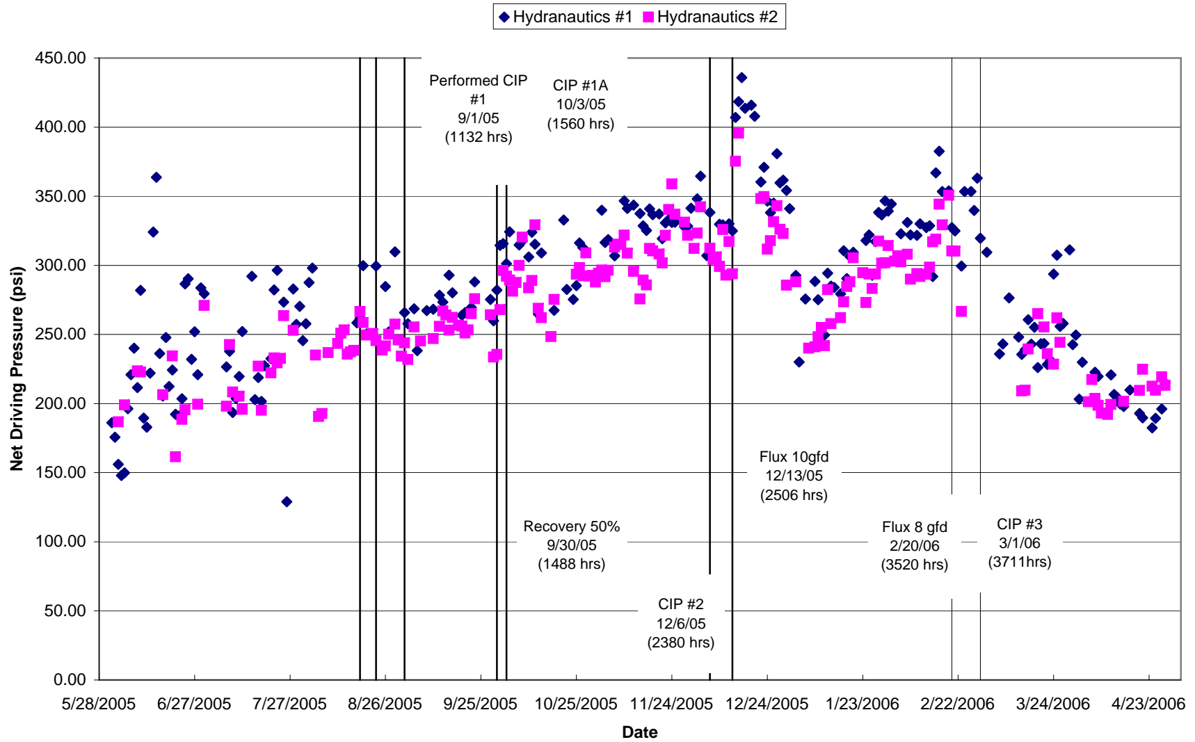
Figure 7.5 MMWD Seawater Desalination Pilot Program SWRO #1 & SWRO #2 Hydranautics Net Driving Pressure
