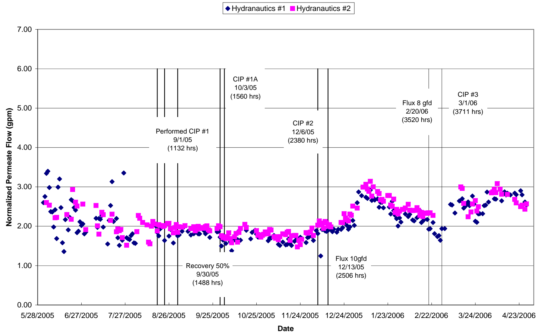
Figure 7.6 MMWD Seawater Desalination Pilot Program SWRO #1 & SWRO #2 Hydranautics Normalized Permeate Flow
