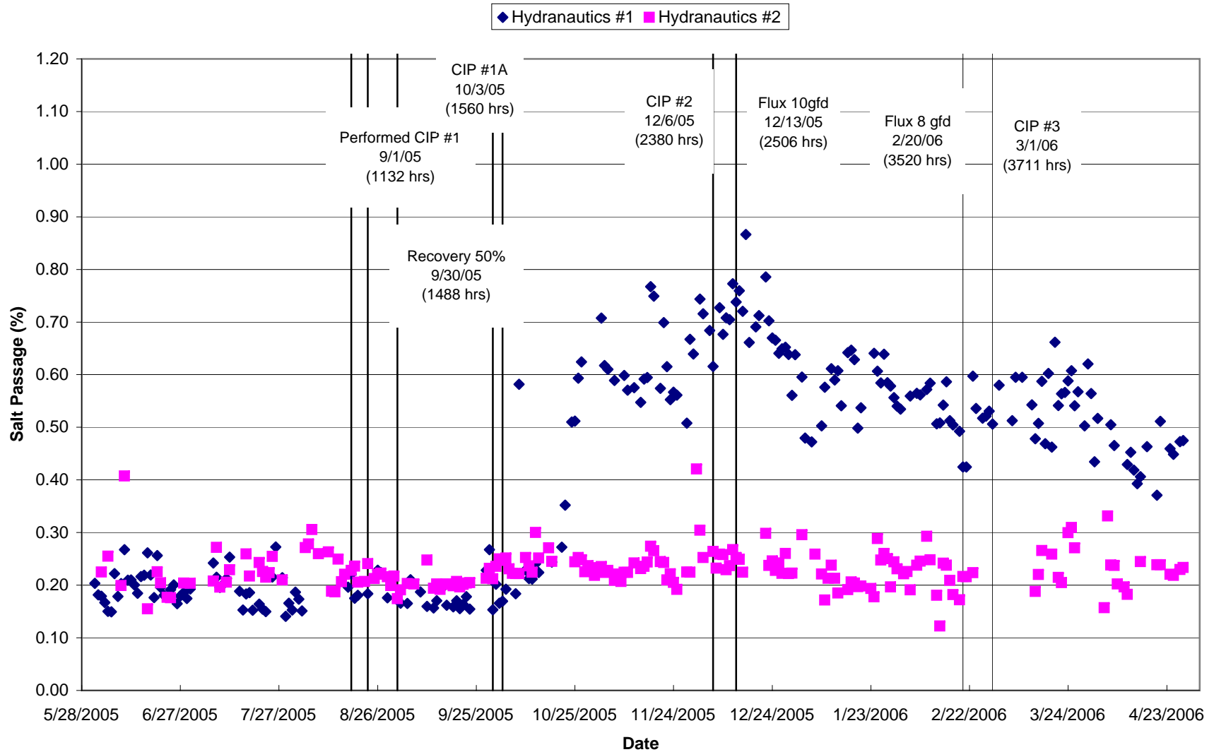
Figure 7.7.1 MMWD Seawater Desalination Pilot Program SWRO #1 & SWRO #2 Hydranautics Normalized Salt Passage
