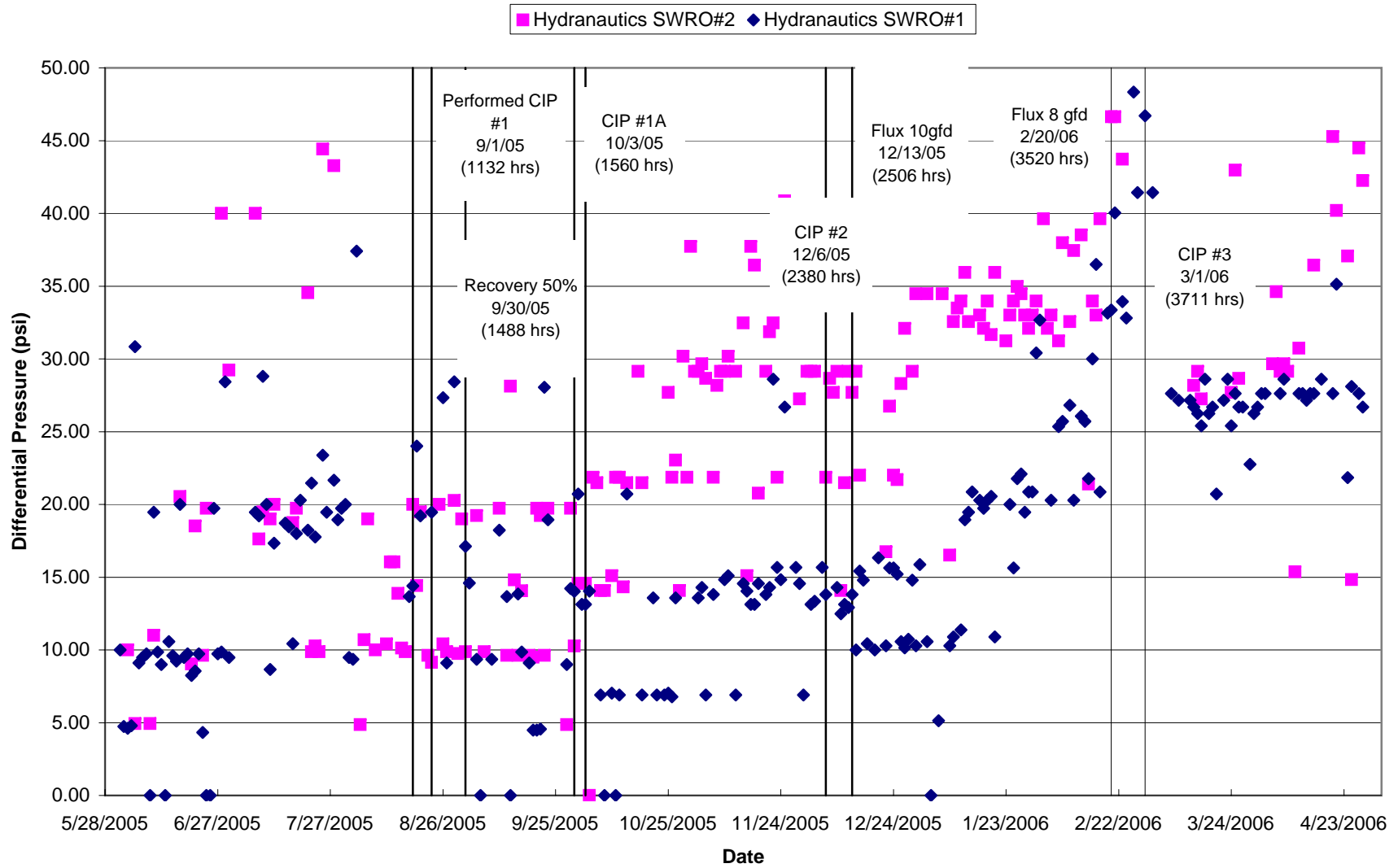
Figure 7.8 MMWD Seawater Desalination Pilot Program SWRO #1& #2 Hydranautics Normalized Feed/Brine Differential Pressure
