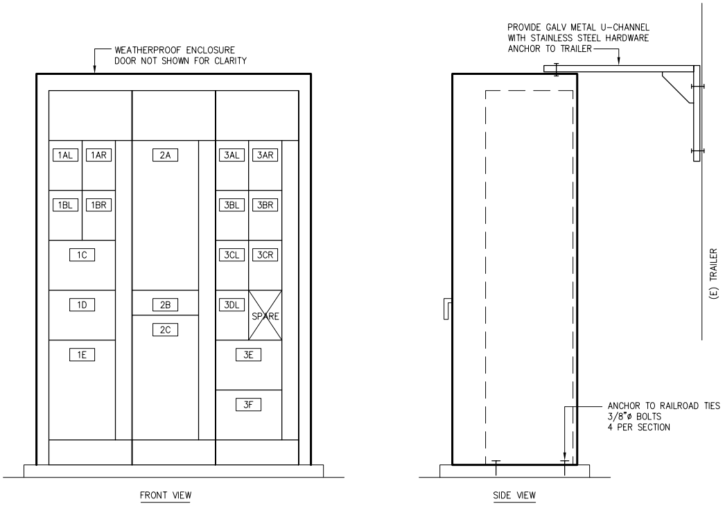
MOTOR CONTROL CENTER ELEVATION SCALE: 3/4" = 1'-0"
