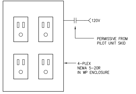
CHEMICAL FEED RECEPTACLE SCALE: NONE
