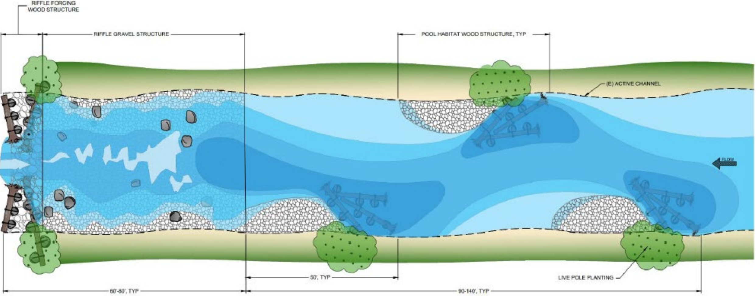
TYPICAL RIFFLE-POOL-WOOD STRUCTURE PLAN VIEW
