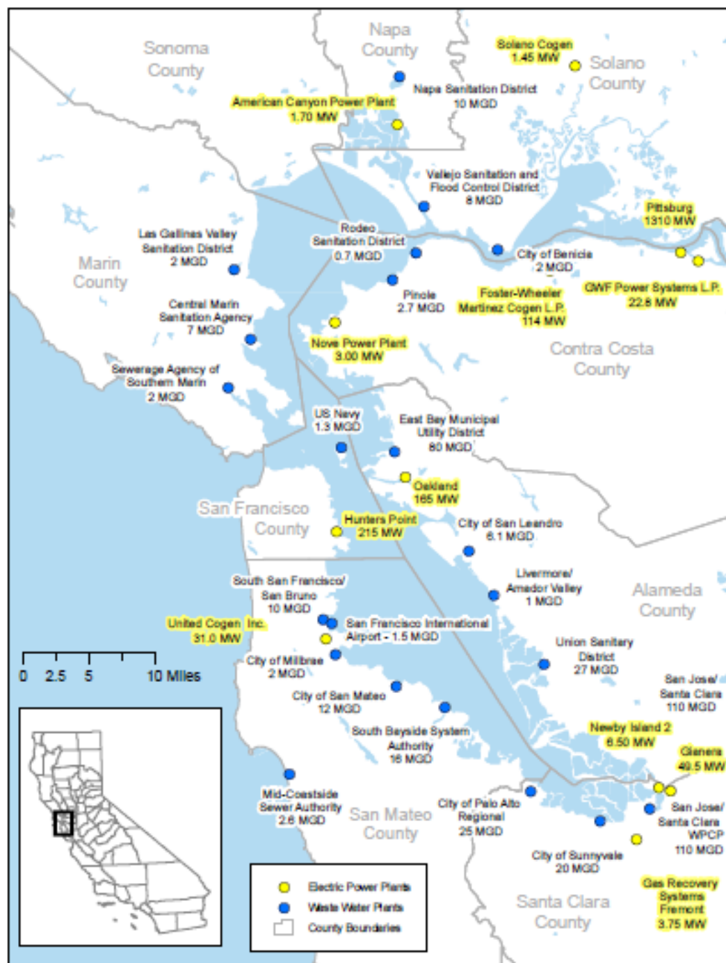
Figure 16-7: Wastewater Treatment Plants and Power Plants on the San Francisco Bay Vulnerable to a 100-Year Flood by 2050
